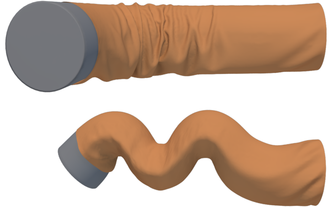
Figure 8: When simulating this cloth with a PSDB featuring only motions in the horizontal plane, our method reproduces plausible wrinkling when bending the left end of the tube to the front (top). When moving to a pose very far from the training data, our solver produces deformations very close to the skinned basis (bottom).
