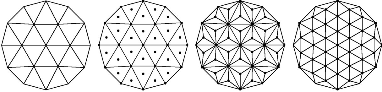
FIGURE 2. \sqrt{3} Subdivision. From left to right: original mesh, added vertices at the midpoints of the faces (step 1), connecting the new points to the original mesh (step 1), flipping the original edges to obtain a new set of faces (step 3). Step 2 involves shifting the original vertices and is not shown.
