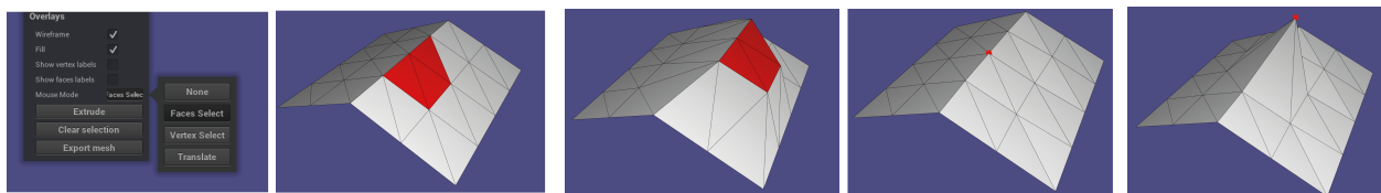
FIGURE 4. Editing operations supported in the code. From left to right: The editor GUI, face selection, face translation, vertex selection, vertex translation.
