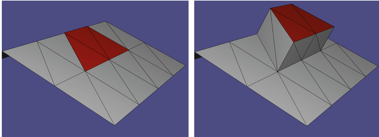
FIGURE 5. Faces extrusion. Left: The user select a set of connected faces. Right: The faces are extruded by their boundary. The boundary vertices/edges are the vertices/edges separating the red selected faces and the unselected grey faces. The boundary vertices are duplicated, the old vertices are slightly translated upwards, and 2 new faces are created for every boundary edge of the selected faces. These faces are connecting the old boundary vertices with the new duplicated ones.
